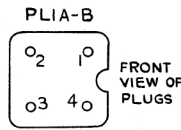
PL3A TO RECEPTION SET R206 PL1B TO A.F.R. No.1
