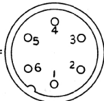
PL3A TO RECEPTION SET R206 PL1B TO A.F.R. No.1
