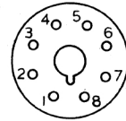
INTERNATIONAL OCTAL V1
