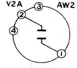
VALVE BASES (VIEWED FROM ABOVE)
