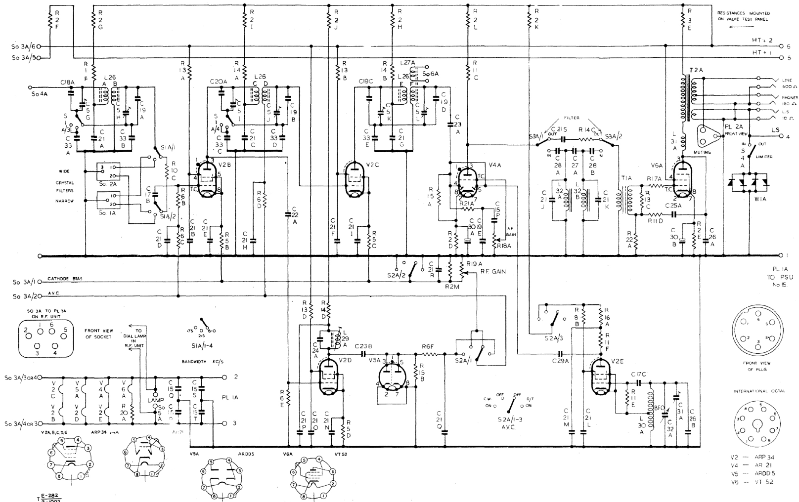
FIG. 8. RECEPTION SET R206. MK.I IF/AF UNIT.
