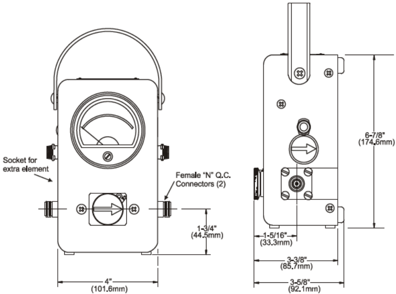
Figure 2 Bird 43 Thru-line Wattmeter Outline Drawing
