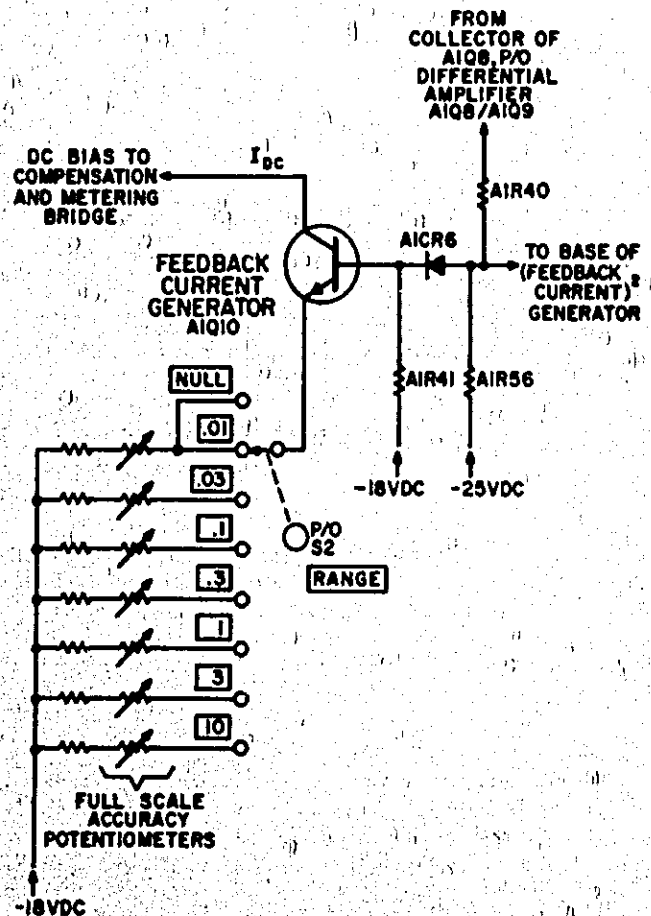
Figure 4-6. Feedback Current Generator
