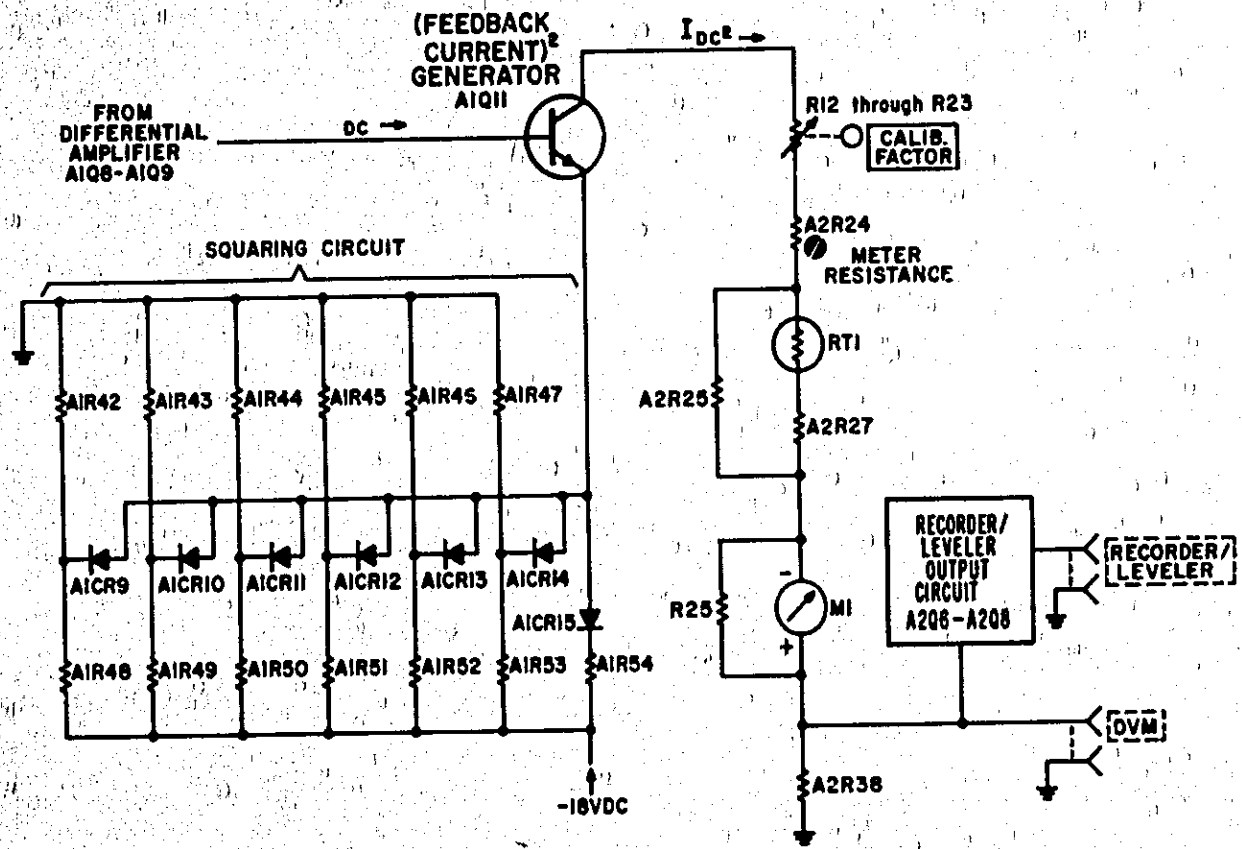
Figure 4-7. Meter Circuit.
