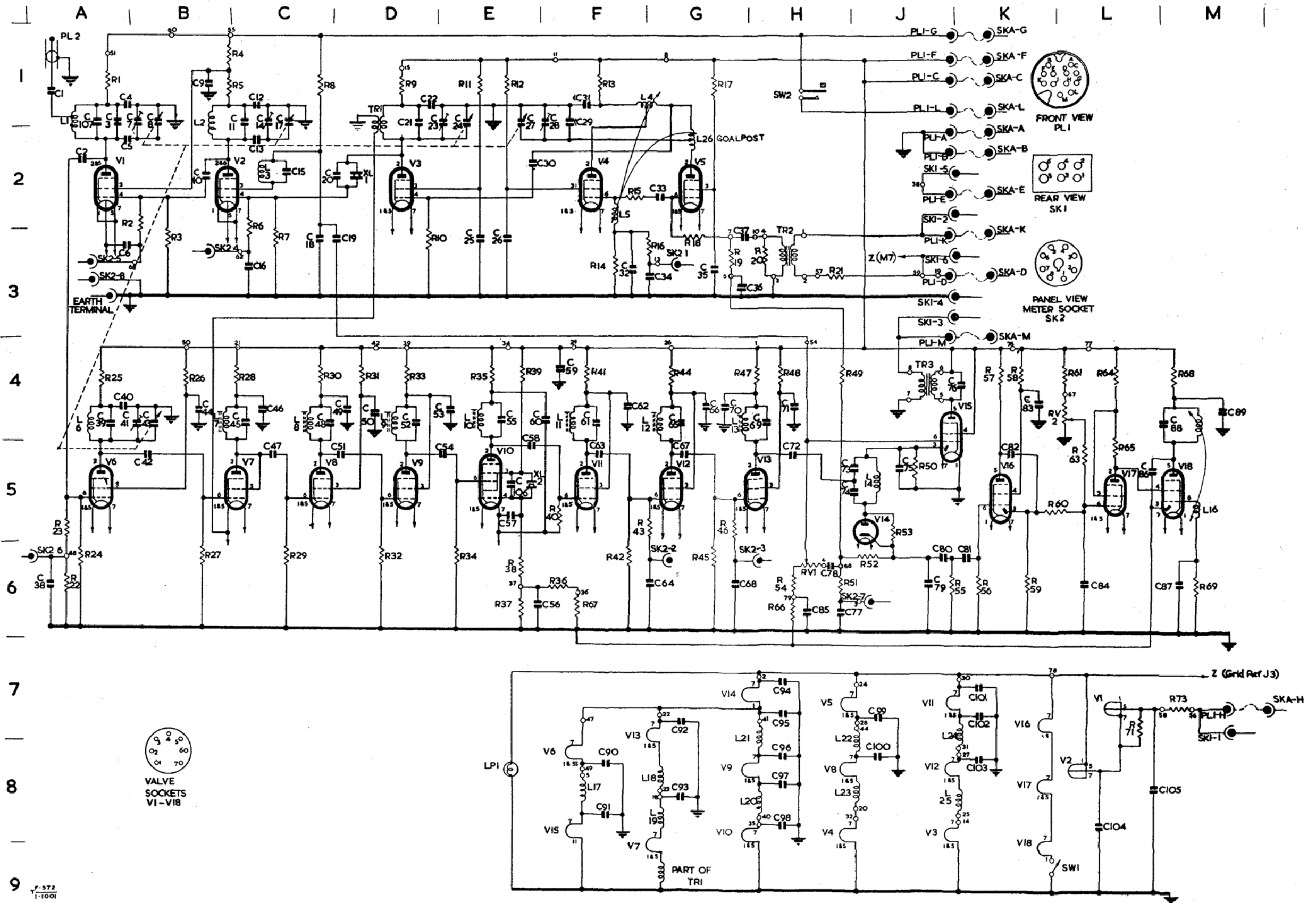
Fig 1001 - Wireless set No. 31 AFV - circuit diagram
